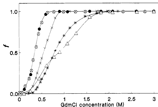
FIGURE 5: Stages of unfolding of staphylococcal \beta -lactamase at 4 °C: (O and ●) fraction of denatured molecules obtained from the enzymatic activity and near UV ellipticity [\theta]_{277} , respectively, by eq 3; (x) fraction of "less compact" molecules obtained from relative areas of corresponding FPLC peaks by eq 1; (*) fraction of unfolded molecules evaluated from the average elution volume \langle V^{el} \rangle by eq 11; (Δ) relative change of far UV ellipticity [\theta]_{220} obtained by eq 12.
